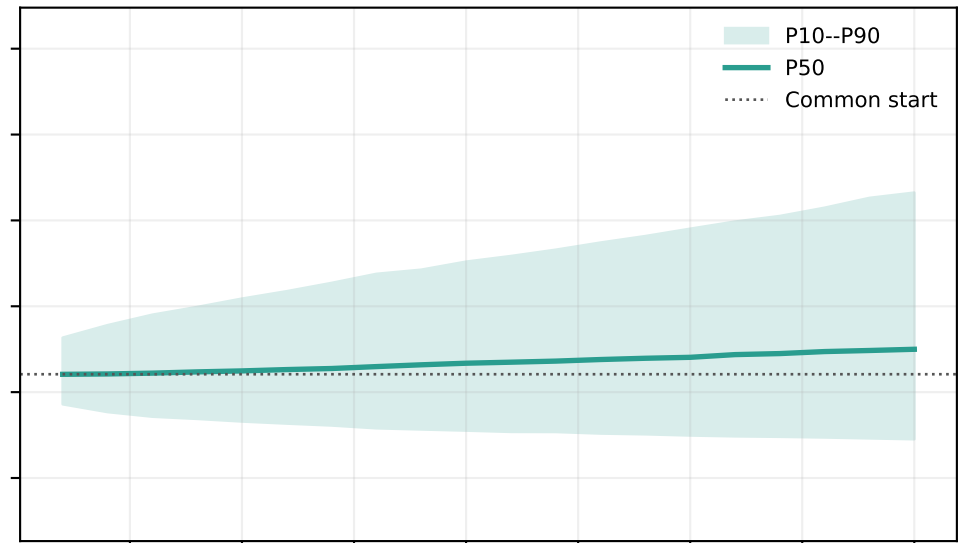
Heston
