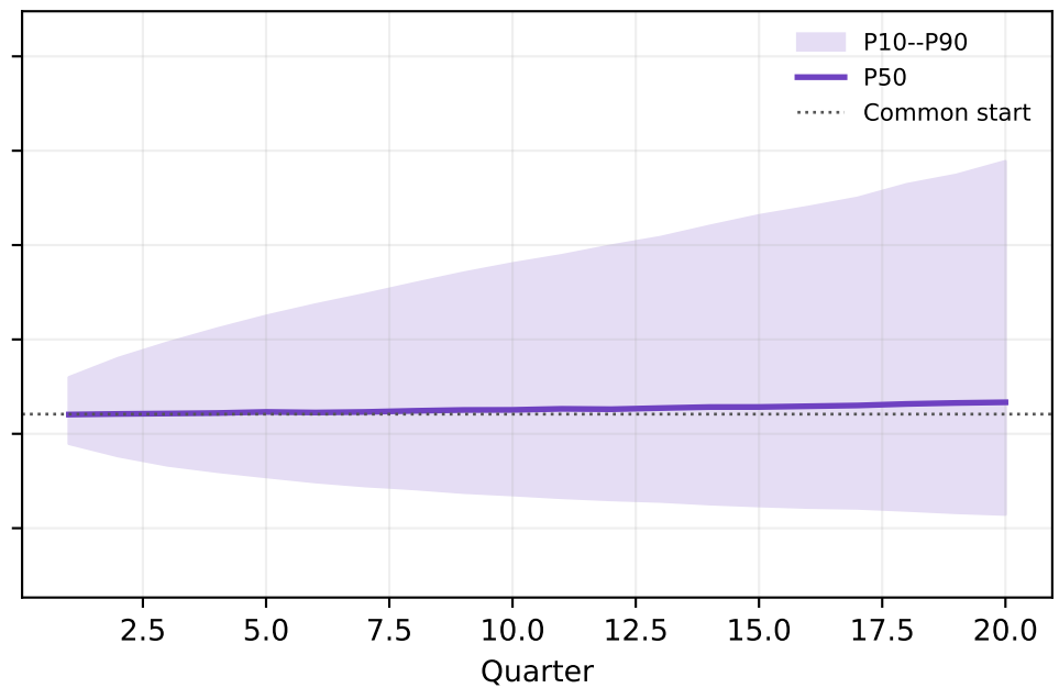
Full Bates-Hawkes
