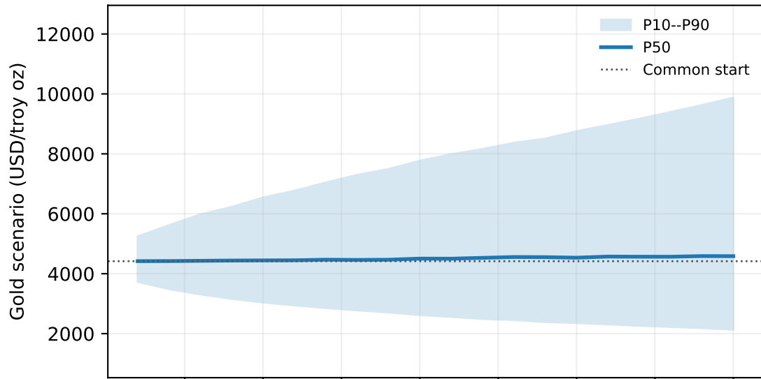
Black-Scholes / GBM
